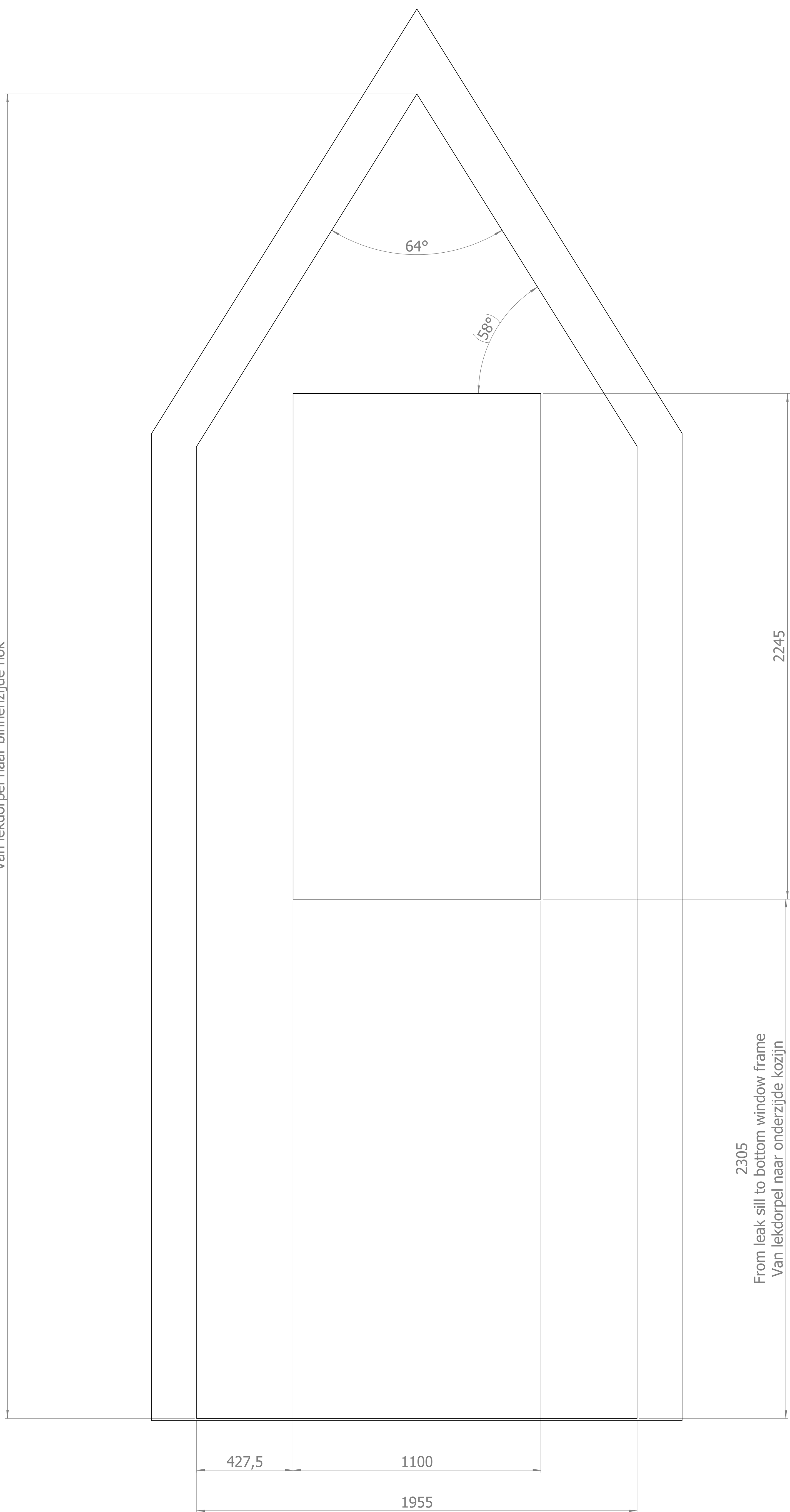
Window Frame (Partial)
