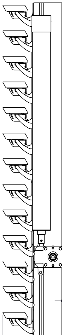
Rackarm 98 mm
